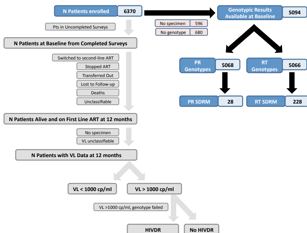
Figure 4.3 Flow diagram of individuals enrolled in WHO surveys of acquired HIV drug resistance: from baseline to 12-month endpoints
