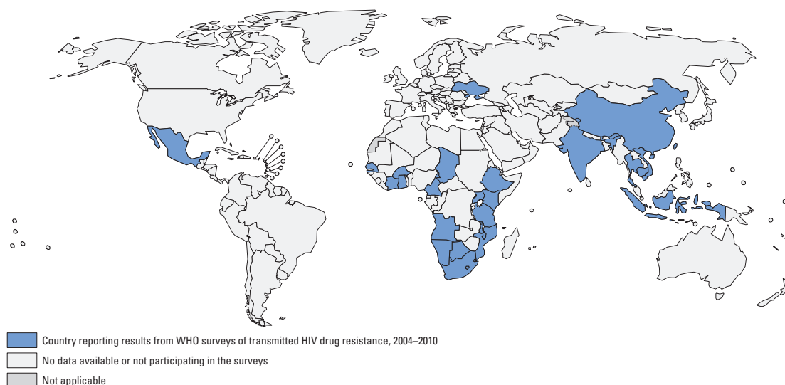
Figure 3.1 Countries (n=26) reporting results from WHO surveys of transmitted HIV drug resistance, 2004–2010
