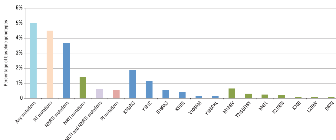
Figure 4.4 Prevalence of HIV drug resistance mutation at baseline in WHO acquired HIV drug resistance surveys
