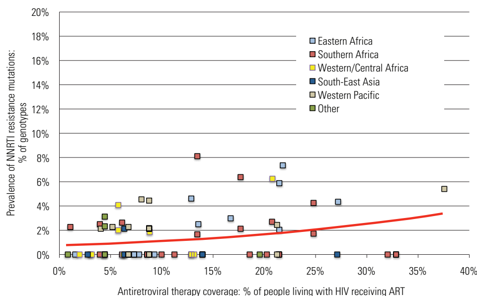
Figure 3.5 Relationship between antiretroviral therapy coverage and prevalence of transmitted NNRTI drug resistance mutations
